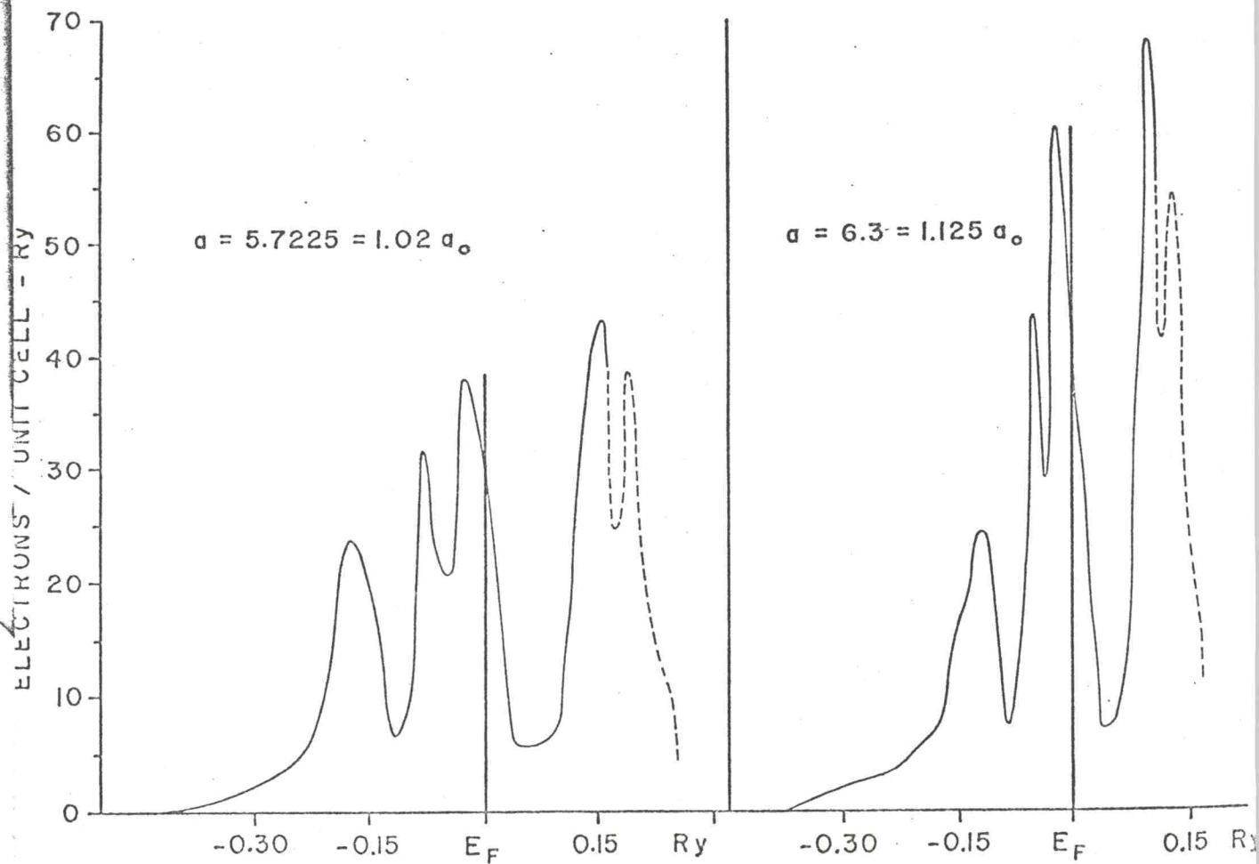
FIG. 6. V densities of states.
